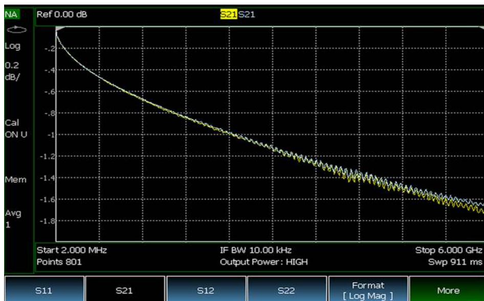
Figure 6. Measurement comparison of a coaxial cable using a Mechanical calibration (blue) and the rapid QuickCal (yellow) available on a FieldFox VNA
