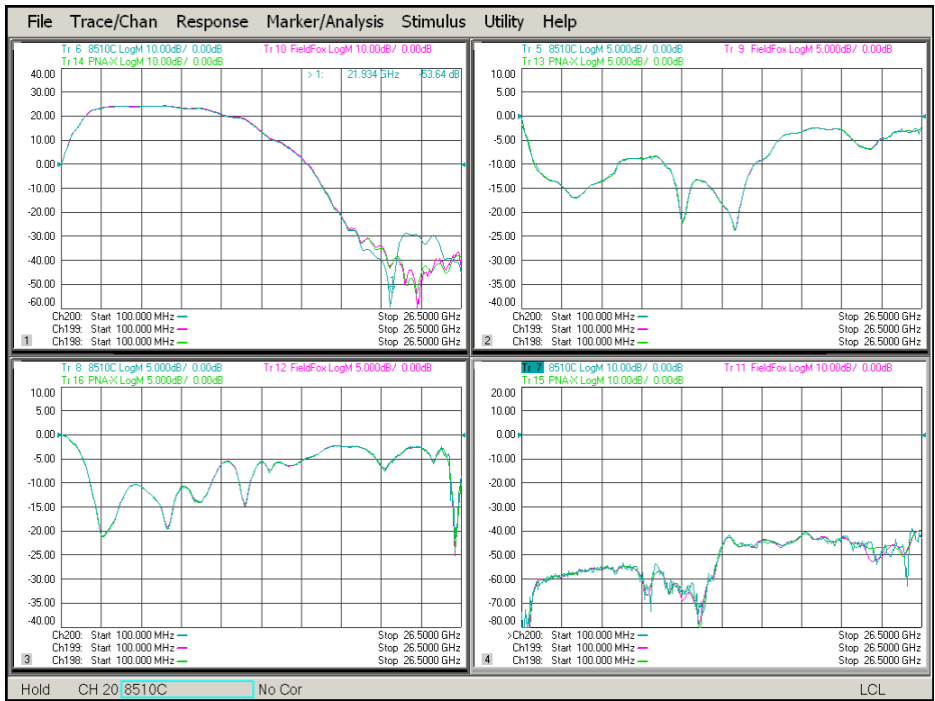
Figure 3. Measured S-parameters of a 3 to 12 GHz broadband amplifier; the plot overlays include measurements from a Keysight 8510C VNA (blue), PNA-X (green) and FieldFox VNA (magenta)
